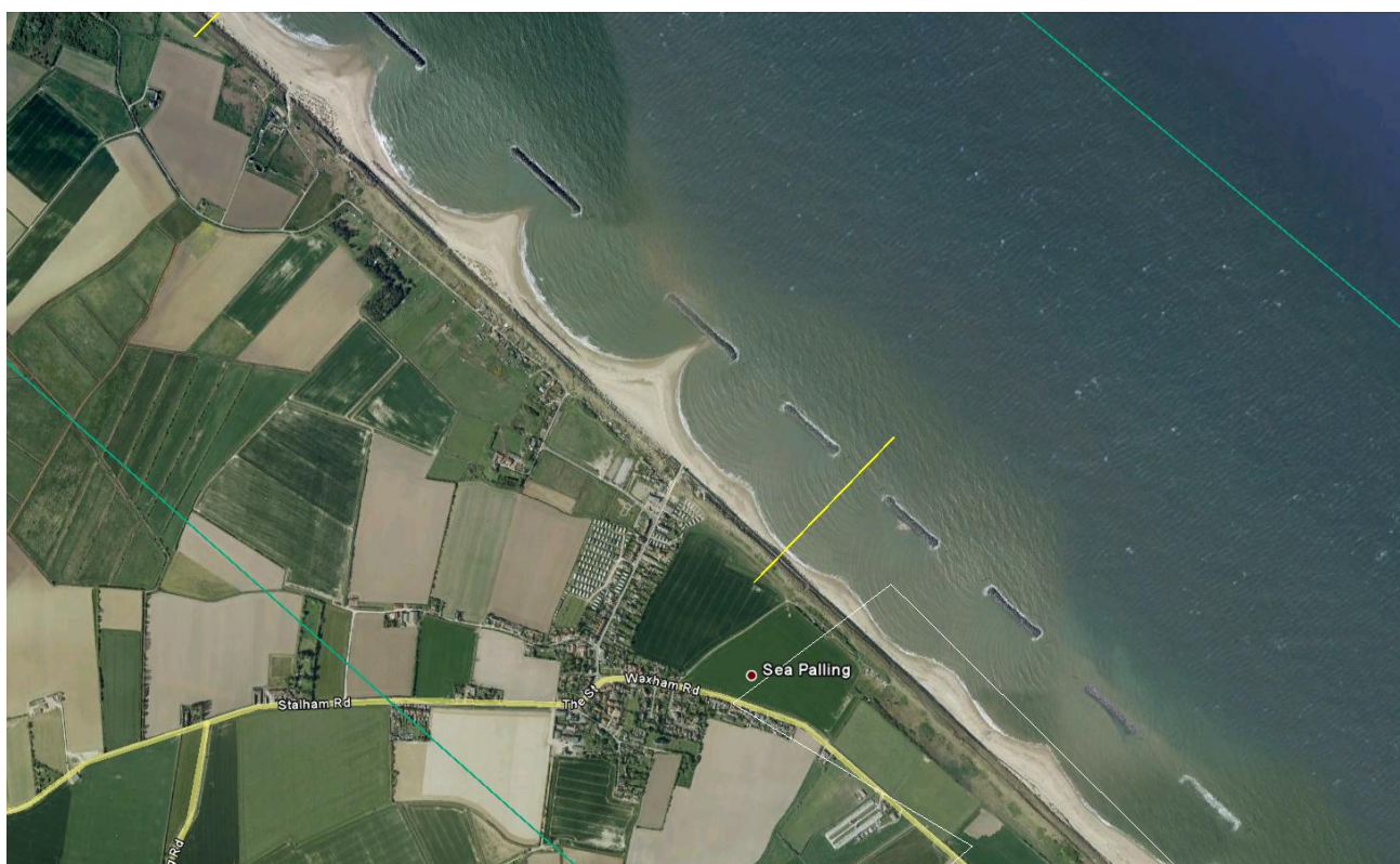
Indicative HDD Alignments for Site 5 (centre) in yellow.
