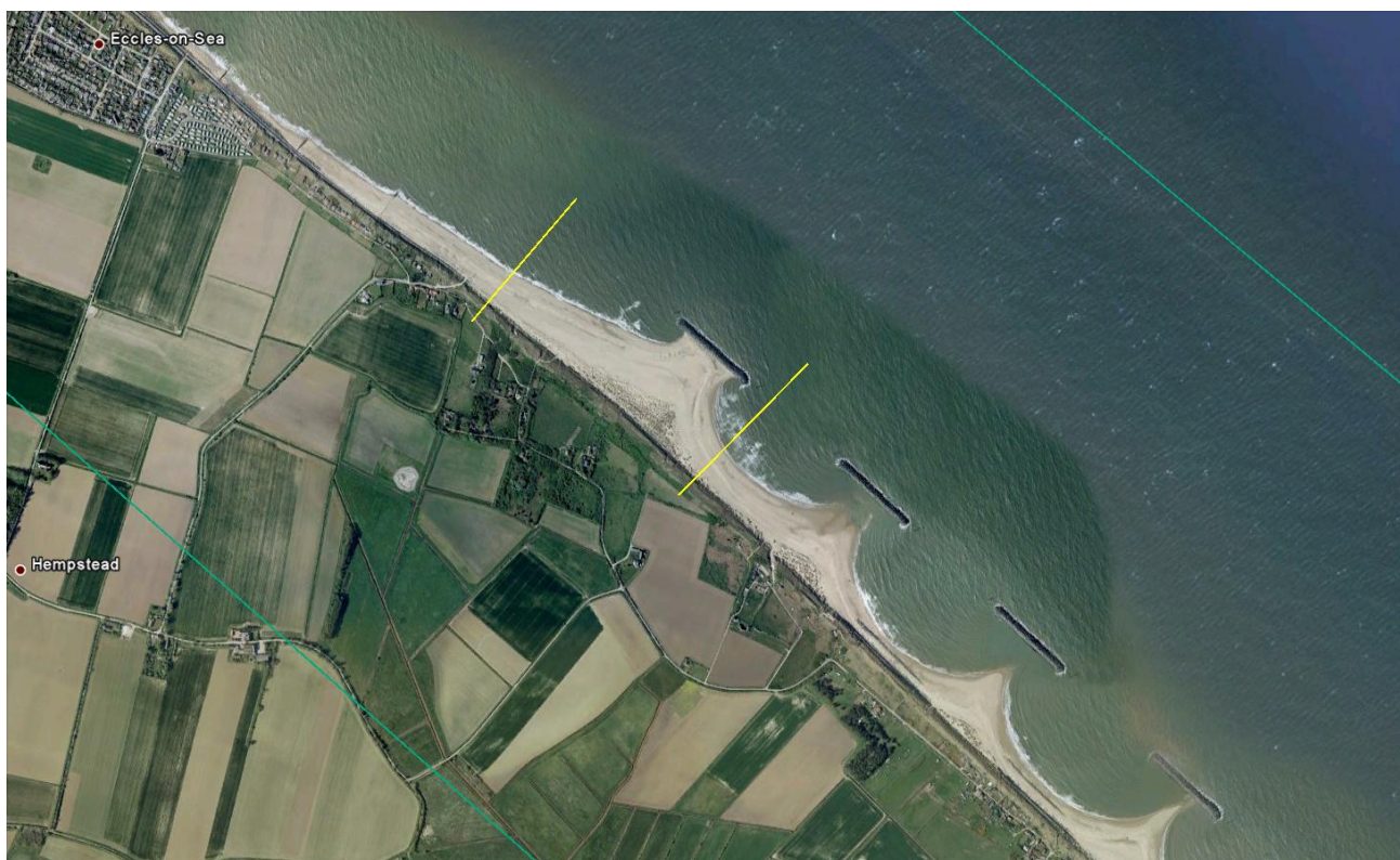
Indicative HDD Alignments for Site 4a (left) and Site 4b (right) in yellow.
