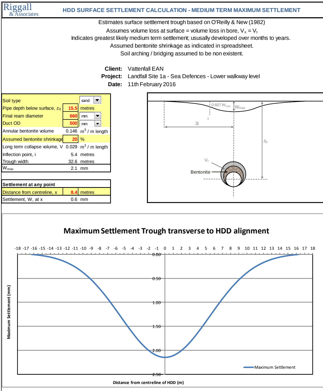
Figure 23. Settlement calculations for lower walkway level of sea defences at Site 1.
