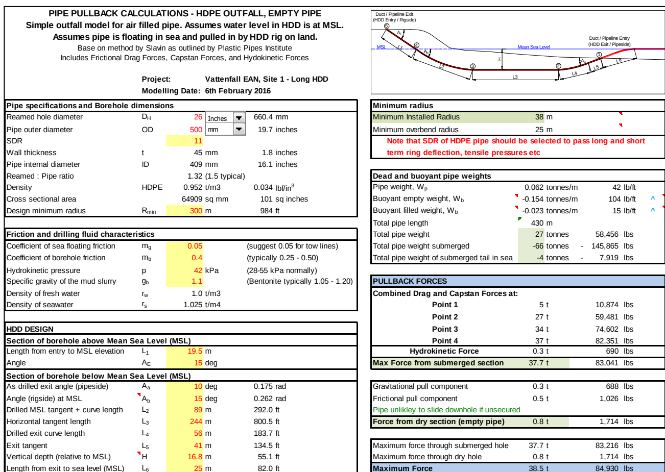
Figure 21. Example calculations for air filled duct installed at Site 1 Long HDD.
