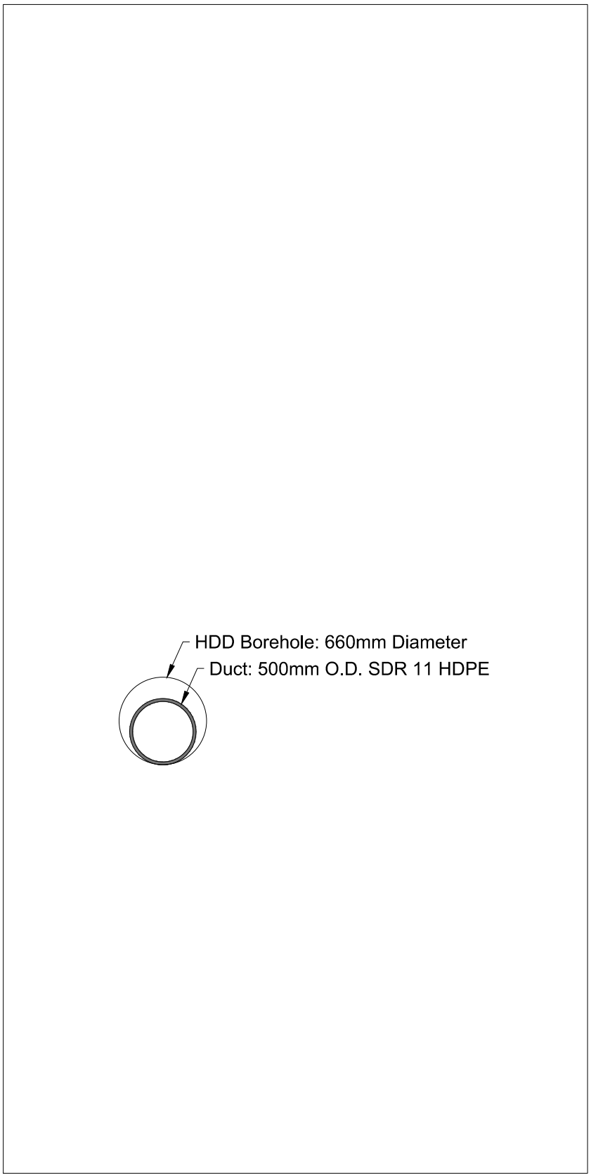
DUCT DETAIL
