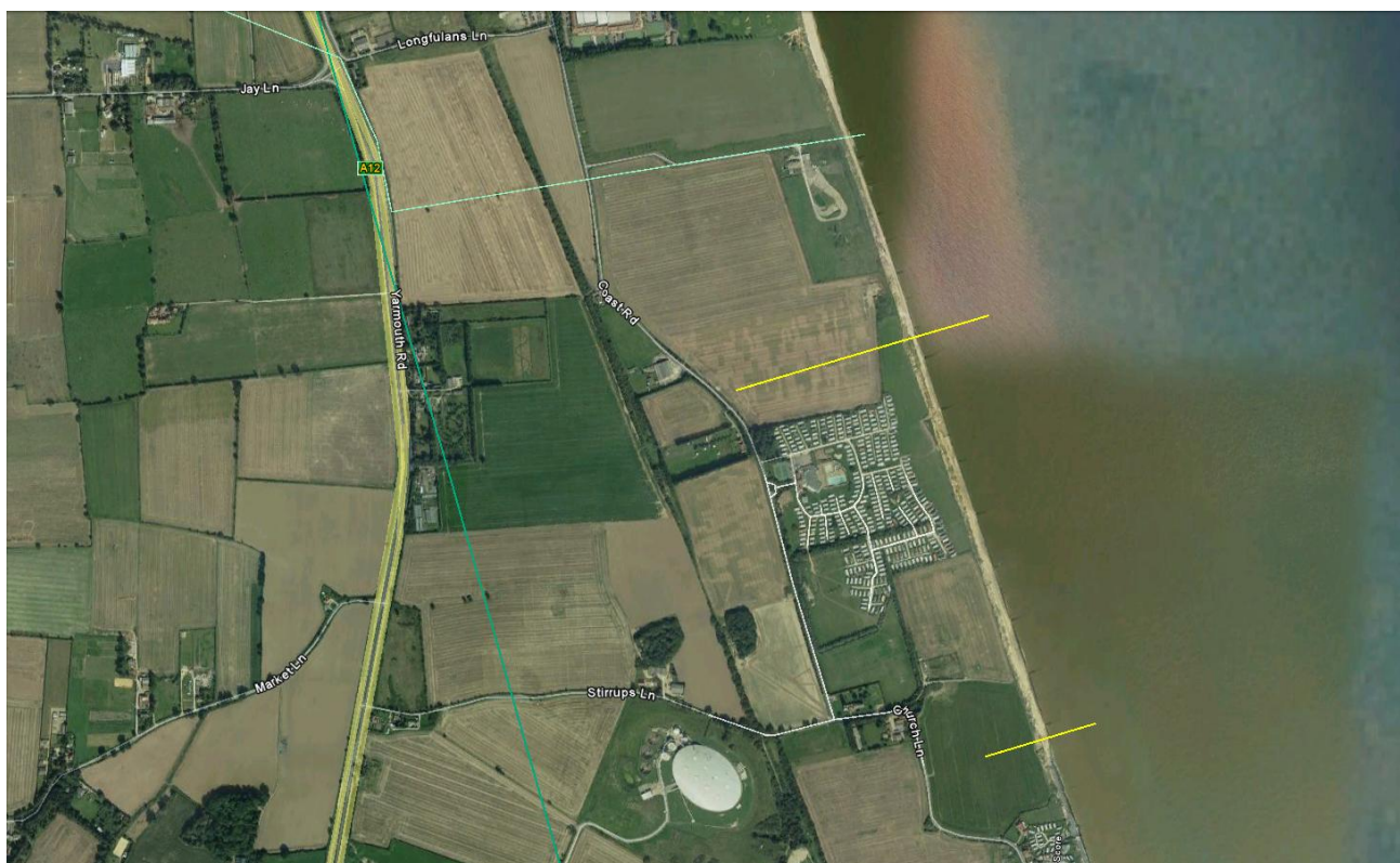
Indicative HDD Alignments for Site 9 (centre) and Site 10 (bottom) in yellow.
